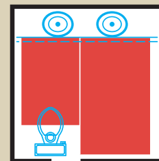
Nuheat Standard Mat
